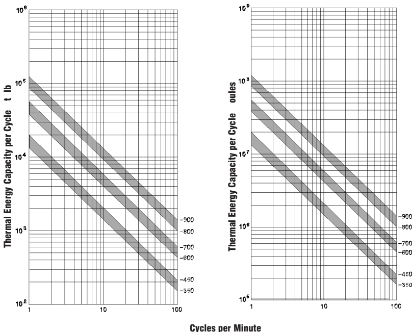
AR and AS Thermal Capacities
